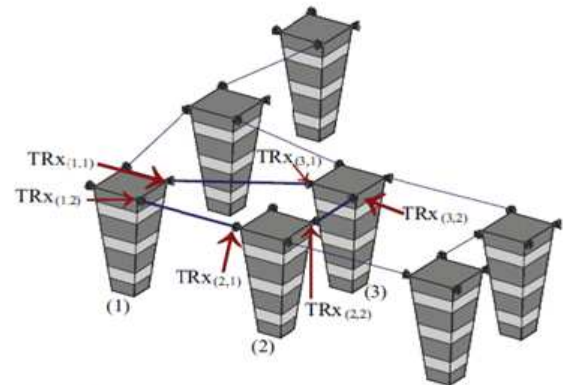
Figure 1: An example of a mesh FSO network. Cooperation is proposed among the transceivers on buildings (1), (2) and (3) where the transceivers on building 2 can help in transmitting an information message from (1) to (3). Note how, given the non-broadcast nature of FSO transmissions, one couple of FSO transceiver units is dedicated for each link.
