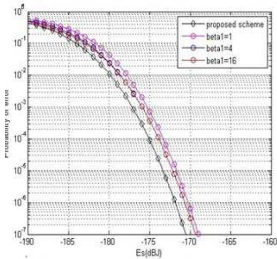
FIGURE 4 PERFORMANCE OF 4-PPM FOR LOGNORMAL FADING CASE(S.I=0.6) WITH NO BACKGROUND RADIATION
