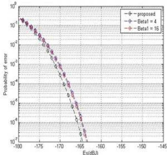
FIGURE 5 PERFORMANCE OF 4-PPM FOR LOGNORMAL FADING CASE (S.I=0.8) WITH BACKGROUND RADIATION
