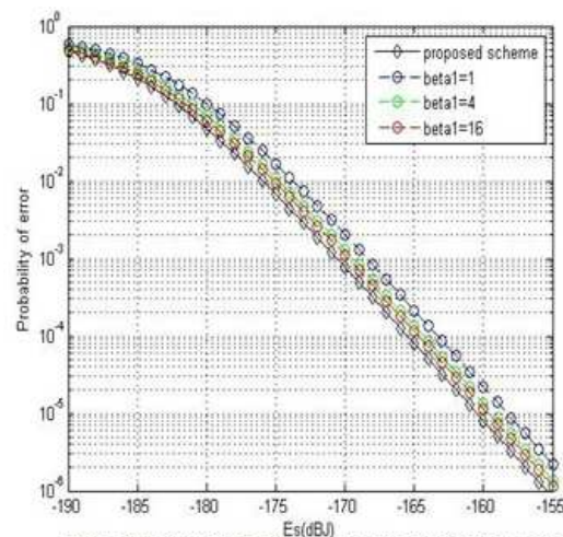
FIGURE 3 PERFORMANCE OF 4-PPM FOR RAYLEIGH FADING CASE WITH NO BACKGROUND RADIATION
