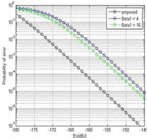
FIGURE 6 PERFORMANCE OF 4-PPM FOR RAYLEIGH FADING CASE WITH BACKGROUND RADIATION
